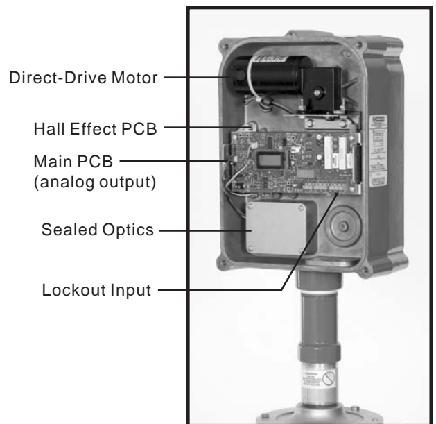
Electronic Compartment
