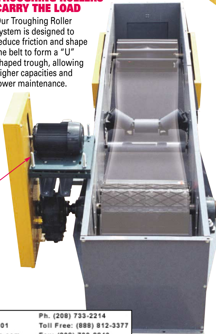
MOTOR AND DRIVE Shown with standard shaft-mounted reducer. Many options available, including right angle, inline, and gear motor drives.
